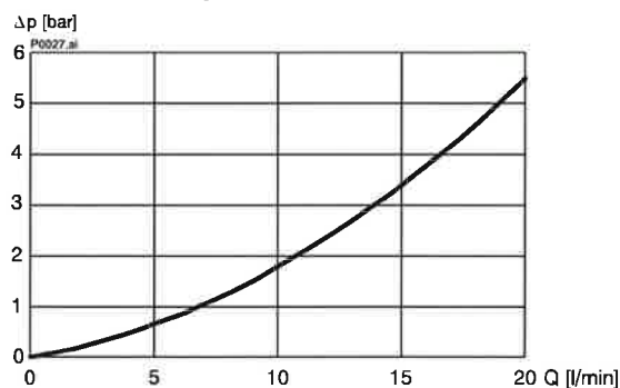
\Delta p = f(Q) Pressure drop - Flow rate characteristic through push-in check valve
