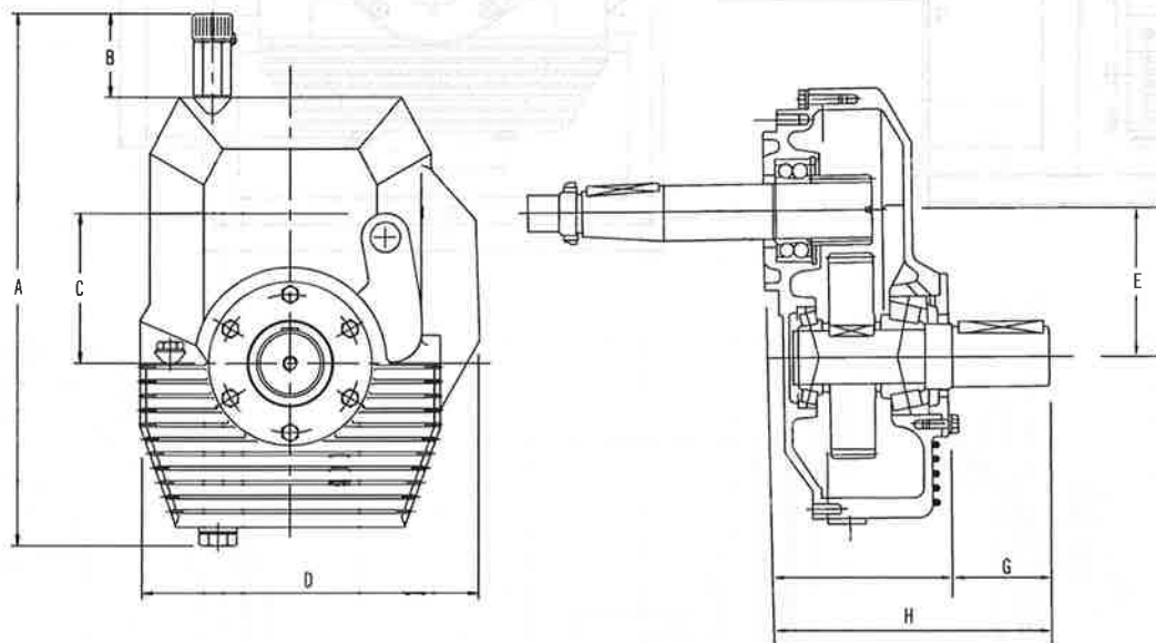
Gearbox Dimensional Data – mm (in)
